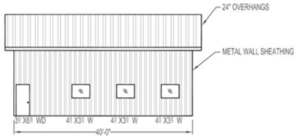
FRONT EAVE
