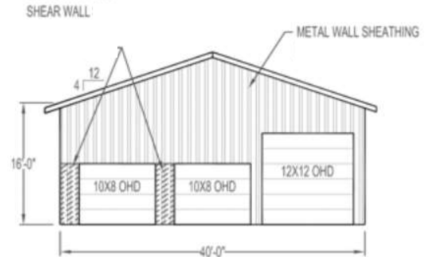
LEFT GABLE
