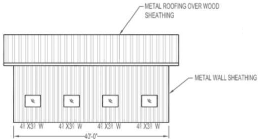
REAR EAVE
